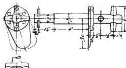
Figs. 3248-3250. Gravity Sander Valve.
